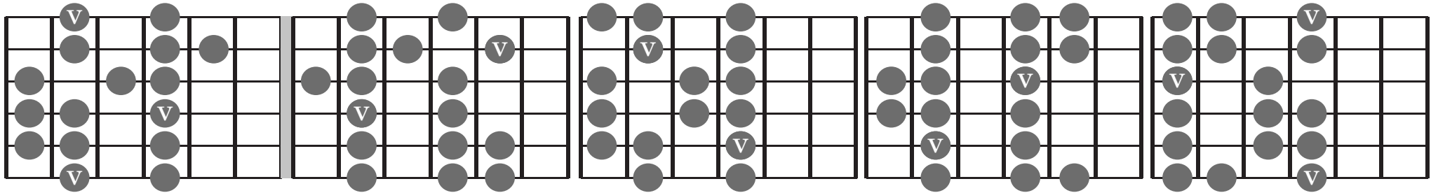
r6 Mixolydian
